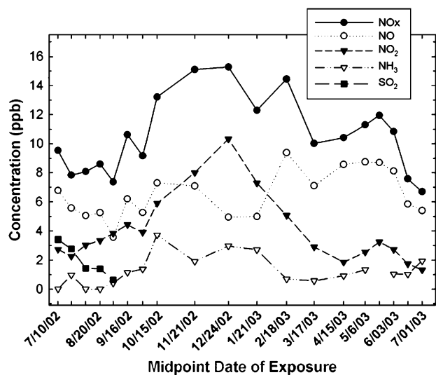
Fig. 6. Average ambient concentrations of \text{NO}_x ( \text{NO}_2 + \text{NO} ), \text{NO}_2 , \text{NO} , \text{NH}_3 , and \text{SO}_2 measured with passive samplers at Horsethief State Park from July 2002–June 2003.
